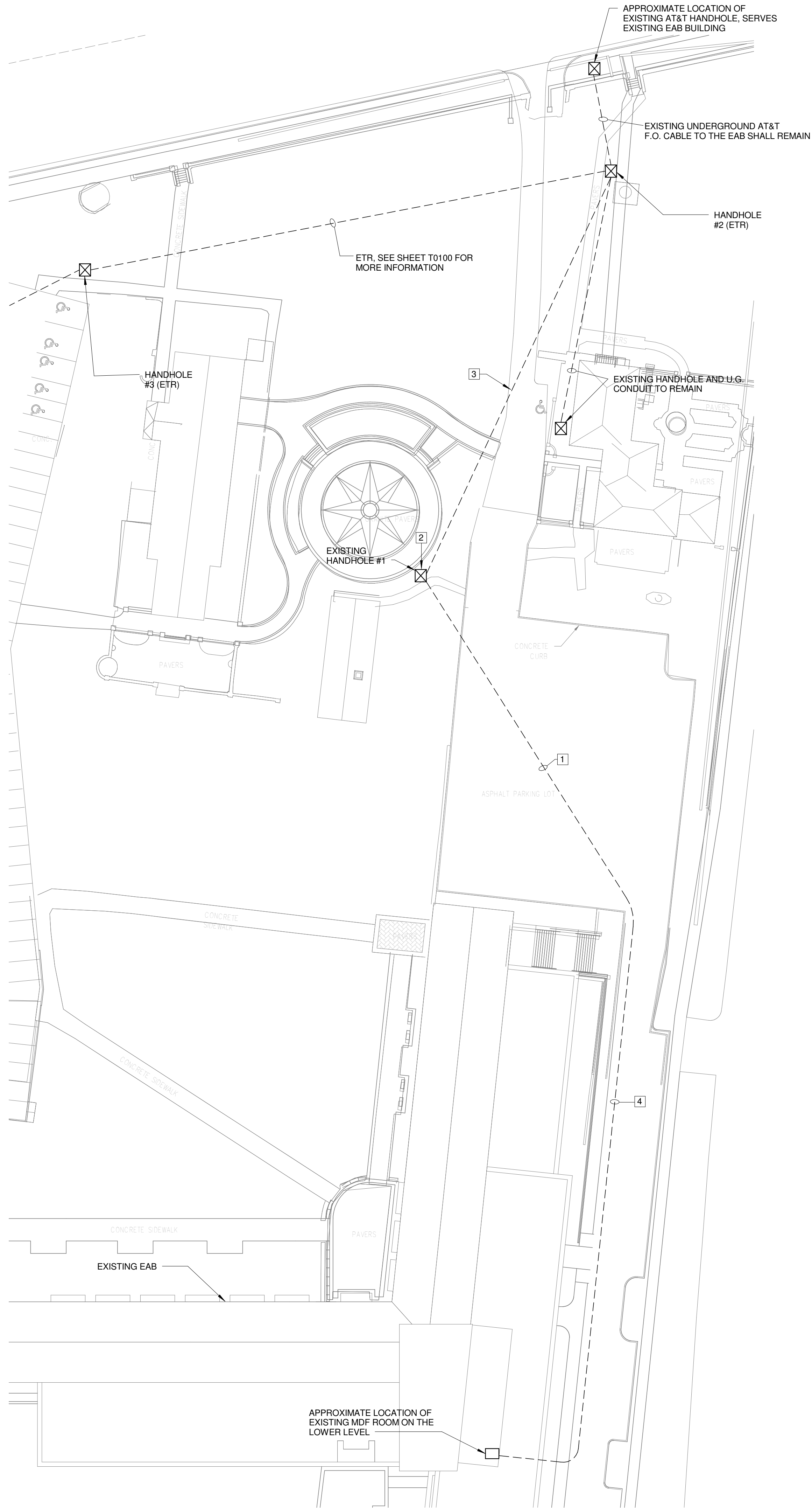
1 TECHNOLOGY SITE PLAN - DEMOLITION 1" = 30'-0"
